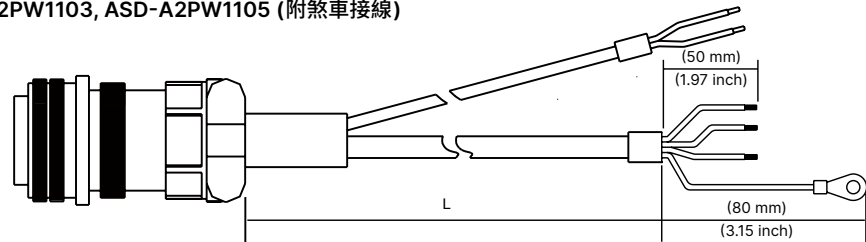
ASD-A2PW1103, ASD-A2PW1105 (附煞車接線)
